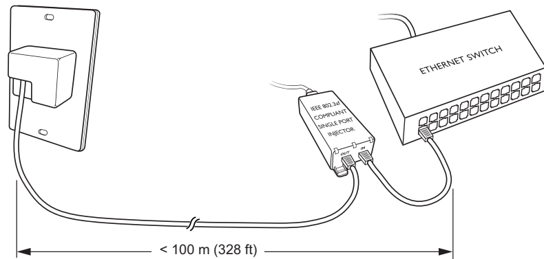
PoE Injector
